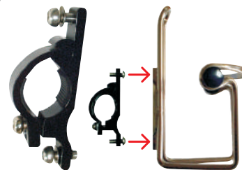
CSC-013 Bracket Material:Alloy Size:Ø22-25.4mm
