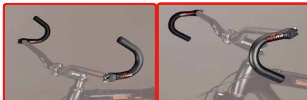
CC-EB12 / CC-EB12S Length 110mm/60mm Weight 155g/121g Material AL6061T6 3D Forged-One Piece Finish Sand Anodized Color
