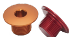
CC-CHB02 For SRAM MTB ■ Material AL7075T6 ■ Length M15 25.8X12.8Lmm ■ Finish Anodized Color
