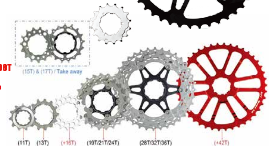
CC-RS42T 40T / 42T +STEEL 16T Rear Sprockets Alloy 7075T6 CNC Thickness 4MM Fits shimano Only
